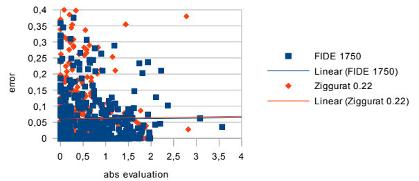
abs evaluation vs avg error (exp scores)
