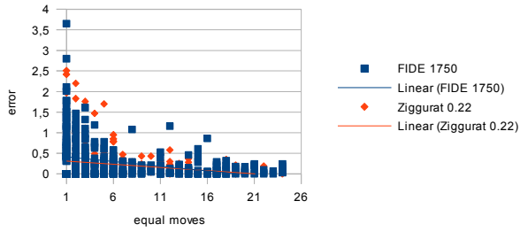
equal moves vs avg error (centipawns)
