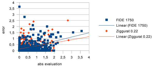
abs evaluation vs avg error (centipawns)
